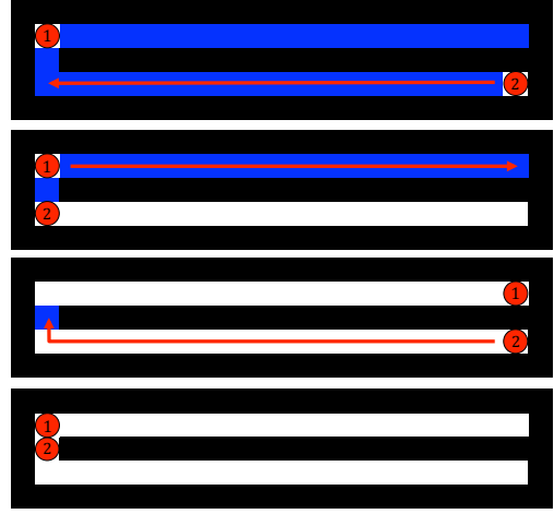
Fig. 4. CLOSESTFRONTIER can be worse than DFS in some cases as well. In this example, using CLOSESTFRONTIER is 1.5\times worse than DFS using only particle 2.
